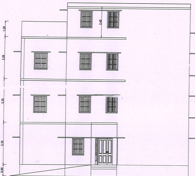
FRONT ELEVATION
