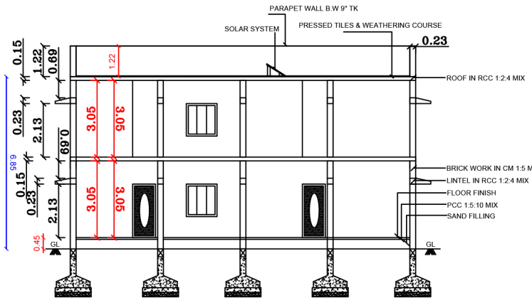
CROSS SECTION AB
