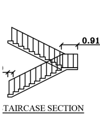
TAIRCASE SECTION
