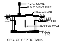
SEC. OF SEPTIC TANK PLAN OF SEPTIC TANK SCALE (1:50)
