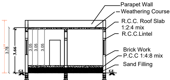
SECTION ON - SD
