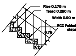
STAIRCASE DETAILS
