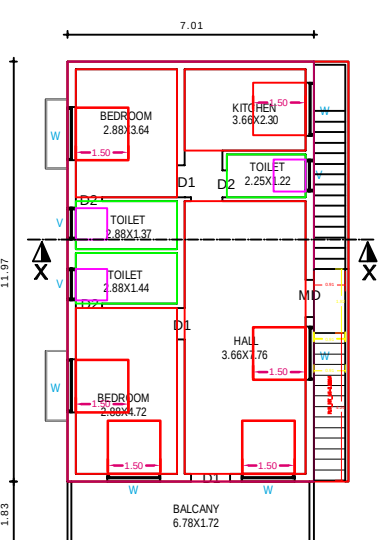
D FIRST FLOOR PLAN
