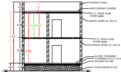
SECTION ON XX
