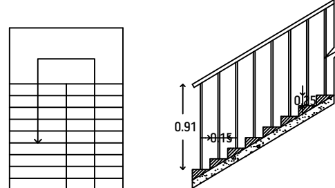
STAIRCASE DETAILS
