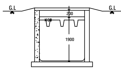
SECTIONAL ELEVATION - BB
