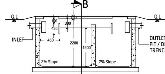
SECTIONAL ELEVATION - AA
