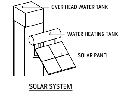
SOLAR SYSTEM
