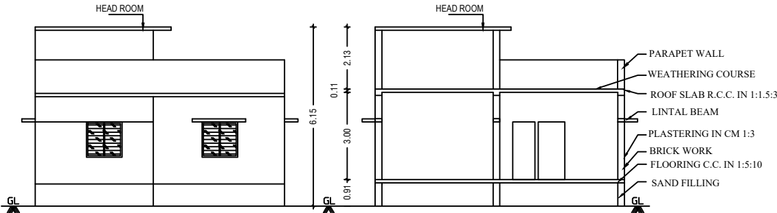
FRONT ELEVATION
