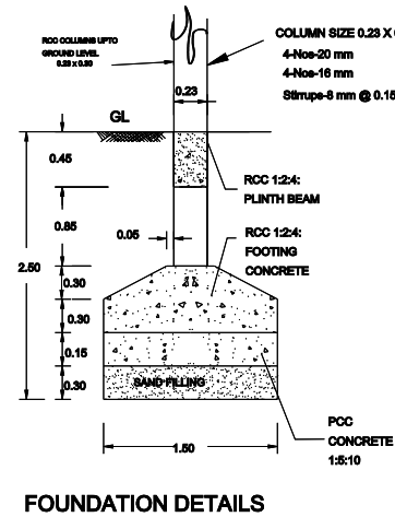
FOUNDATION DETAILS
