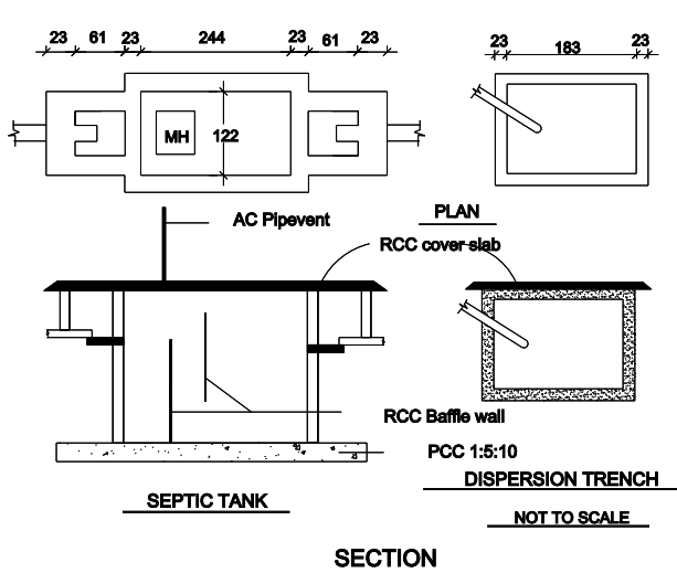
SECTION
