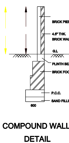
COMPOUND WALL DETAIL
