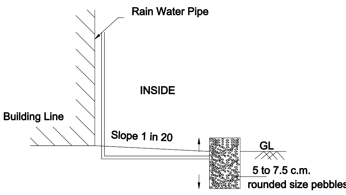
RAINWATER HARVESTING
