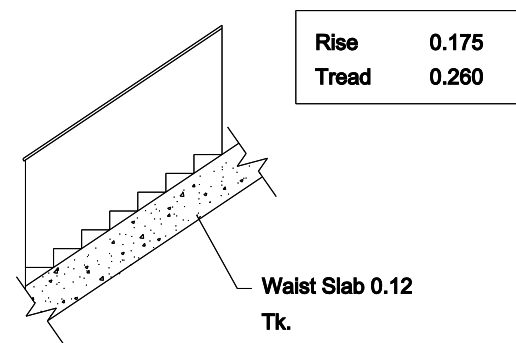
Staircase Details
