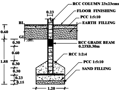
FOUNDATION DETAILS
