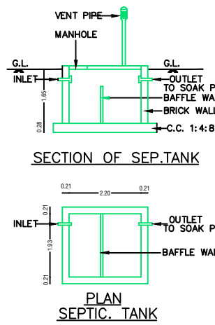
PLAN SEPTIC. TANK
