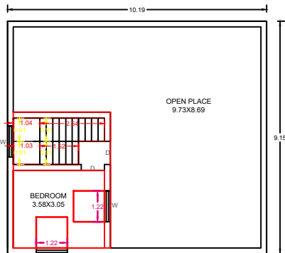
PRO.FIRST FLOOR
