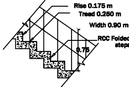
STAIRCASE DETAILS
