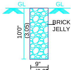
PERCOLATION PIT
