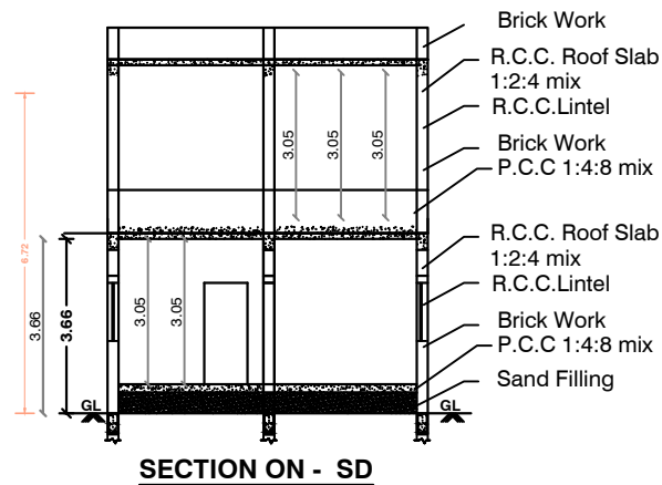
SECTION ON - SD
