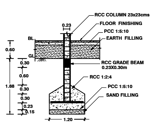
FOUNDATION DETAILS
