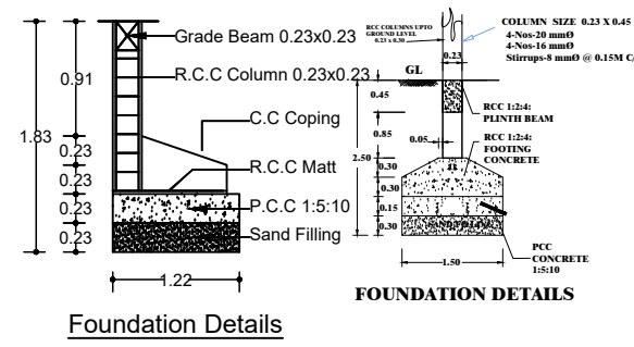
Foundation Details
