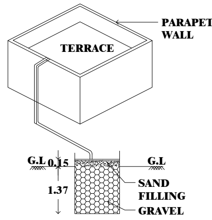
COLLECTION SUMP FOR HARVESTING FOR TERRACE
