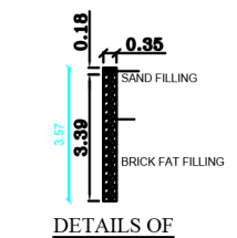
DETAILS OF PERCOLATION PIT RWHL_CAPACITY_L=1000 LTRS
