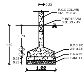
COLUMN FOUNDATION DETAILS
