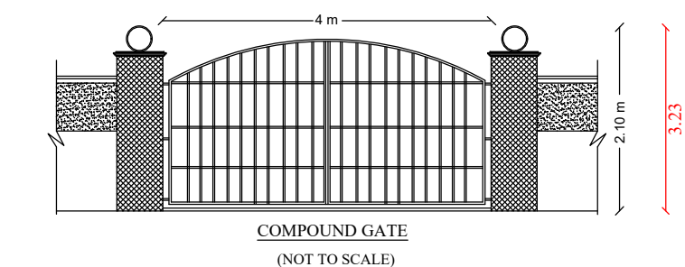
COMPOUND GATE (NOT TO SCALE)
