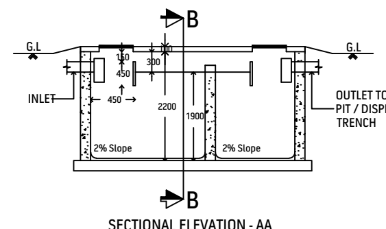
SECTIONAL ELEVATION - AA
