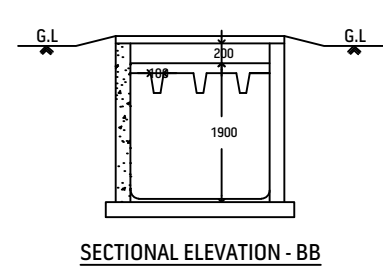
SECTIONAL ELEVATION - BB
