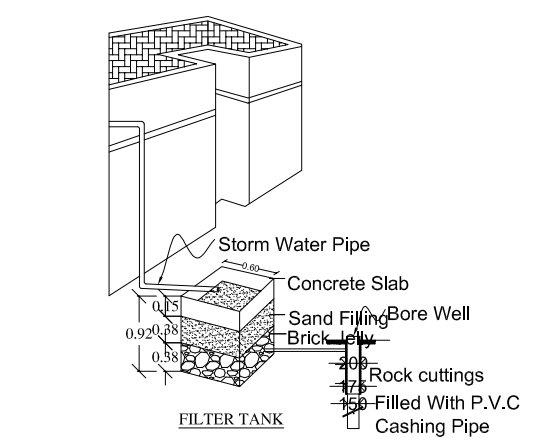
RAIN WATER STORAGE ARRANGEMENTS
