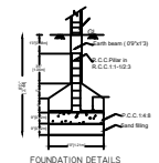
FOUNDATION DETAILS
