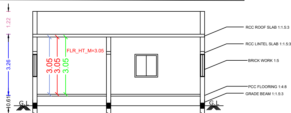
SECTION AT AB
