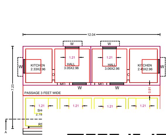
FLOOR PLAN
