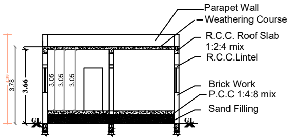
SECTION ON - SD
