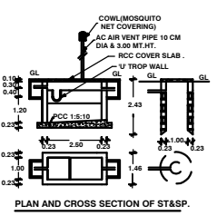
PLAN AND CROSS SECTION OF ST&SP.
