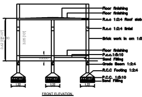
FRONT ELEVATION
