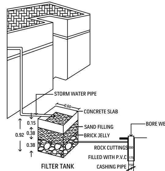
RAIN WATER STORAGE ARRANGEMENTS
