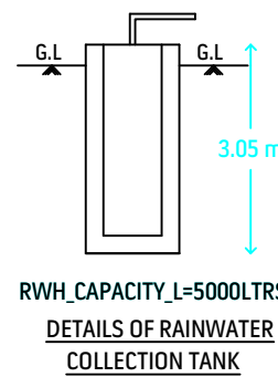
DETAILS OF RAINWATER COLLECTION TANK
