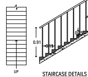
STAIRCASE DETAILS
