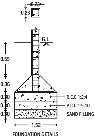
FOUNDATION DETAILS
