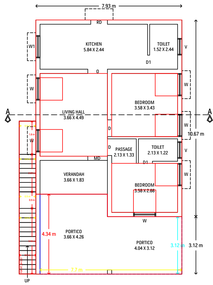
EXISTING & ADDITION GROUND FLOOR PLAN
