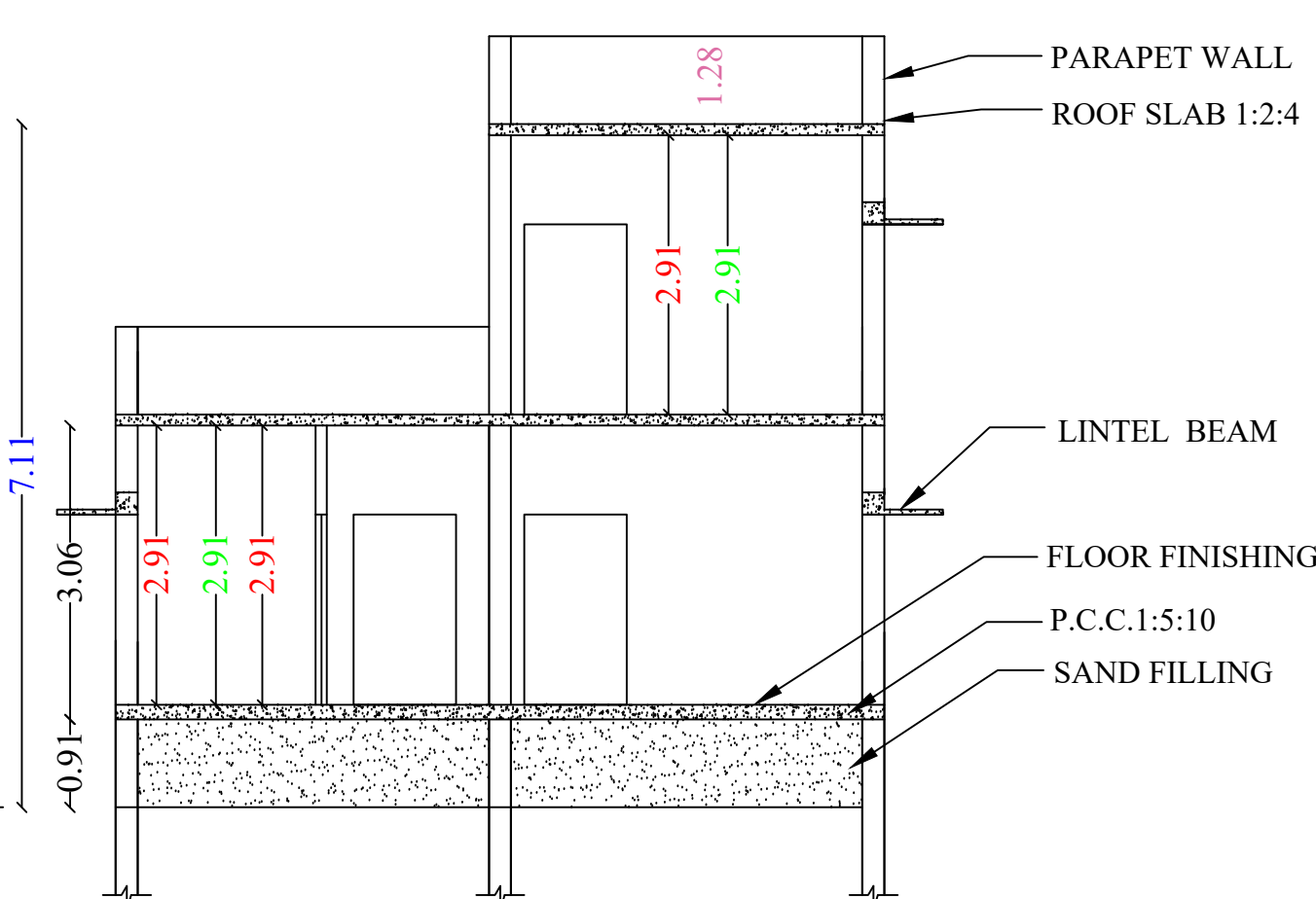
SECTION ON X-Y
