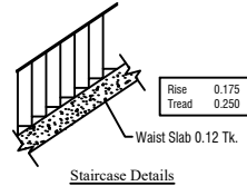
Staircase Details
