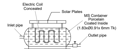
Solar water heater
