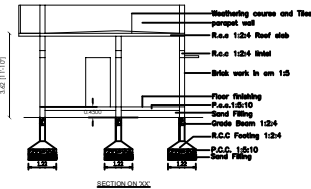
SECTION ON X-X'
