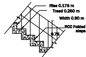
STAIRCASE DETAILS
