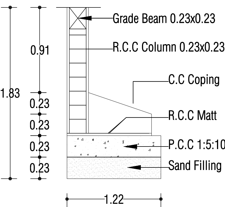
Foundation Details
