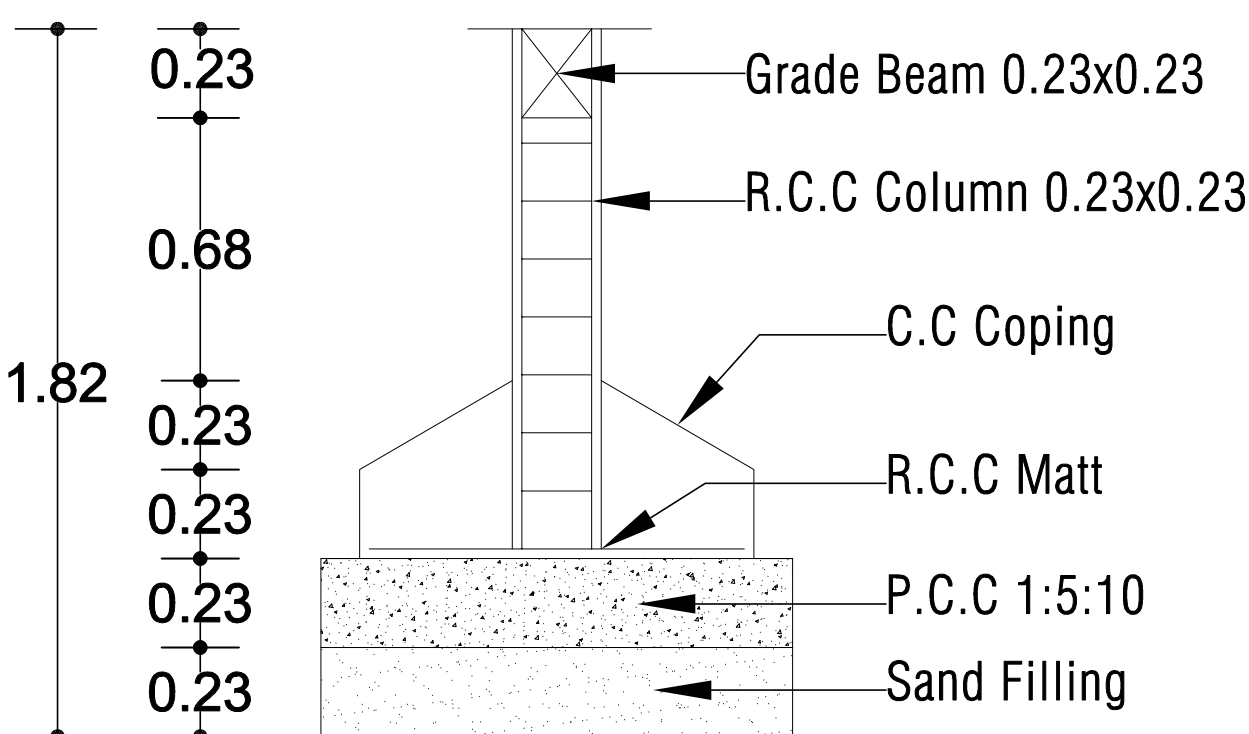
Foundation Detail
