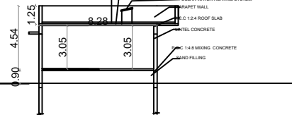
SECTION ON-AA'
