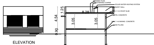
SECTION ON-AA'
