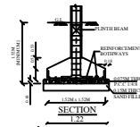
FOUNDATION DETAILS
