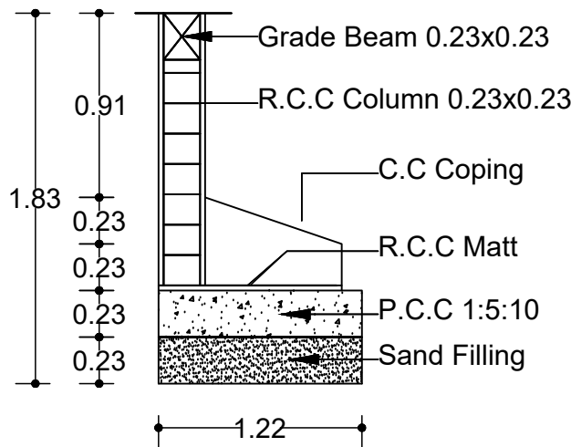
Foundation Details
