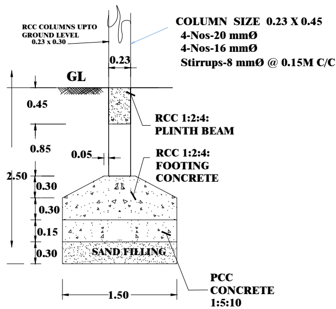
FOUNDATION DETAILS
