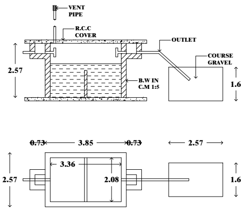
SEPTIC TANK & D-TRENCH DETAILS [ NOT TO SCALE ]
