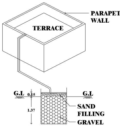
COLLECTION SUMP FOR HARVESTING FOR TERRACE
