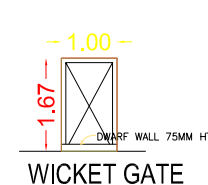
WICKET GATE
