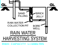
RAIN WATER HARVESTING SYSTEM RWH_CAPACITY_L=1000LTRS
