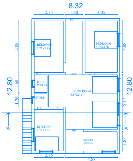
FLOOR PLAN
