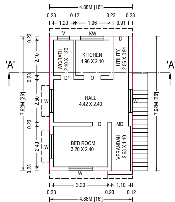
FLOOR PLAN
