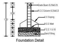
Foundation Detail
