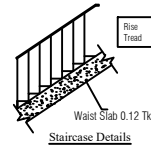
Staircase Details
