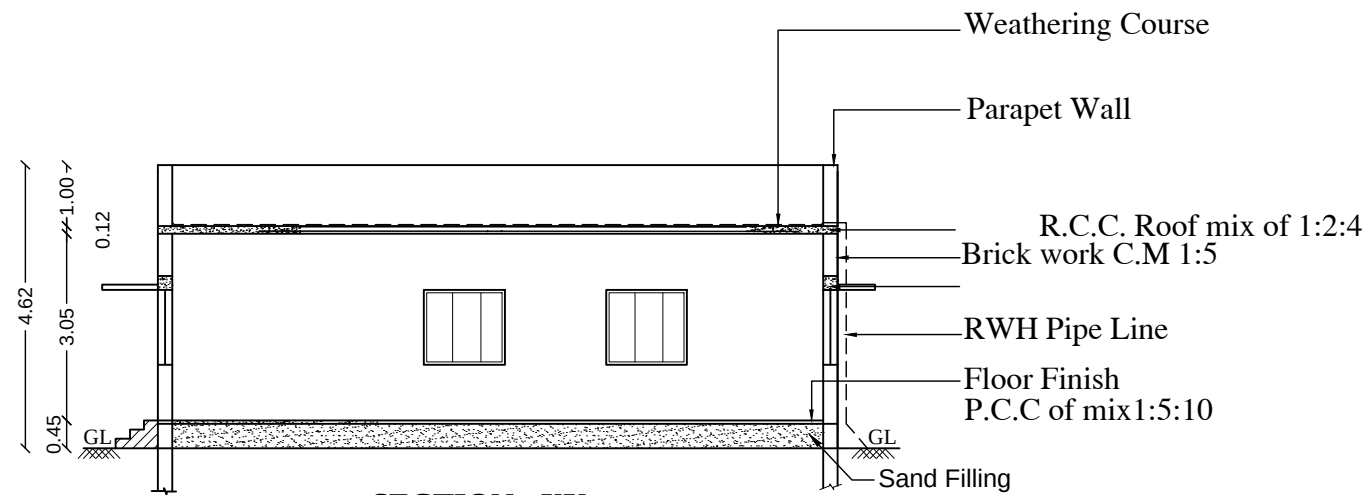
SECTION - XY
