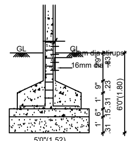
COLUMN FOUNDATION DETAIL SCALE (1:50)
