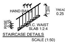
STAIRCASE DETAILS SCALE (1:50)
