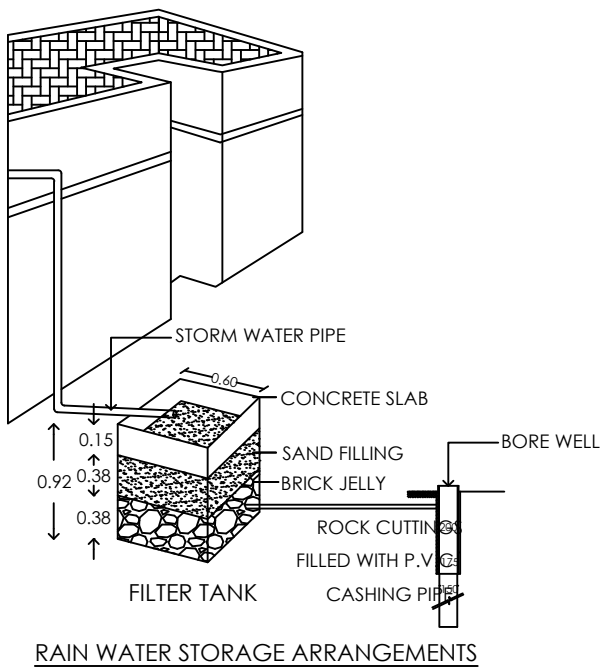
RAIN WATER STORAGE ARRANGEMENTS
