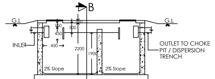
SECTIONAL ELEVATION - AA
