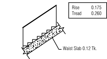
Staircase Details
