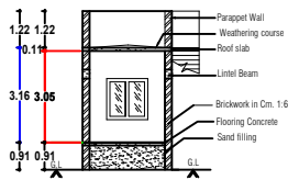
SECTION ON 'AB'
