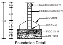
Foundation Detail
