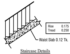
Staircase Details
