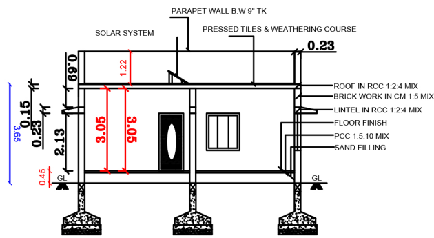
CROSS SECTION AB
