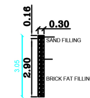
DETAILS OF PERCOLATION PIT RWL_CAPACITY_L=1000 LTRS
