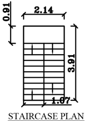
STAIRCASE PLAN
