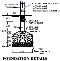
FOUNDATION DETAILS
