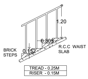
STAIRCASE DETAILS [NTS]
