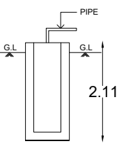
RWH_CAPACITY_L=5000LTRS DETAILS OF RAINWATER COLLECTION TANK
