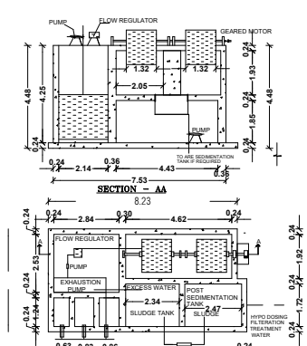
SEWAGE TREATMENT PLANT (S.T.P.) WASTE WATER FILTRATION BY RECIRCULATION SYSTEM G.O(MS) NO.136 DT:11.10.02
