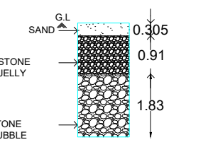
RAINWATER HARVESTING PIT [RWHP]
