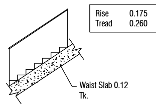
Staircase Details
