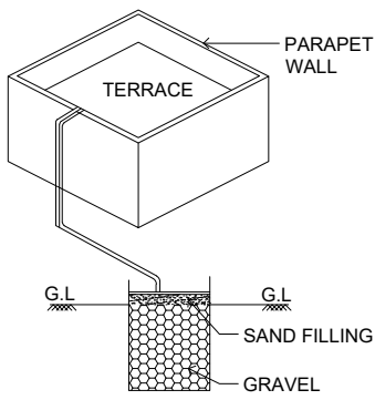
COLLECTION SUMP FOR HARVESTING FOR TERRACE
