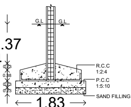
COLUMN DETAILS [ NOT TO SCALE ]
