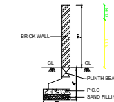
COMPOUND WALL DETAIL
