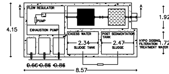
SEWAGE TREATMENT PLANT [S.T.P.] WASTER WATER FILTRATION BY RECIRCULATION SYSTEM G.O[MS] NO.138 DT:11-10-02 SCALE : 1:100
