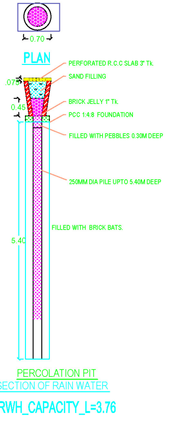
PERCOLATION PIT SECTION OF RAIN WATER RW[CAPACITY]_L=3.76
