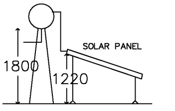
SIDE ELEVATION [ Not to scale ]
