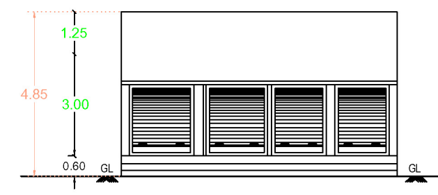
FRONT ELEVATION
